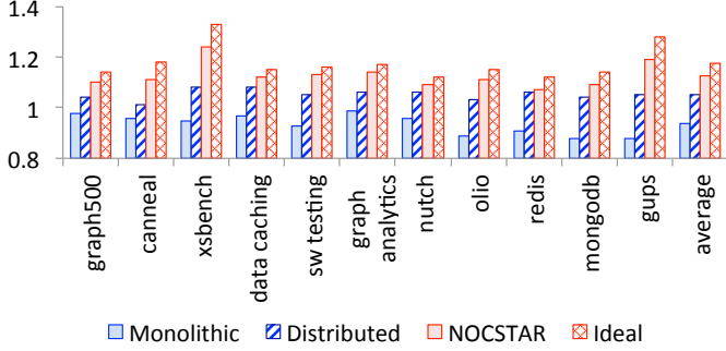
Fig. 12: Speedups for monolithic, distributed, and NOCSTAR compared to ideal case with zero interconnect latency to the shared L2 TLB. Results assume 16-core Haswell systems using only 4KB pages.
