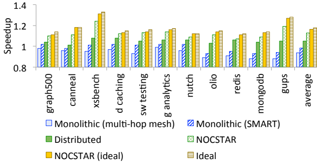
Fig. 15: Speedup over baseline configuration with private L2 TLBs. We show two monolithic approaches (with traditional multi-hop mesh and SMART, as well as an ideal NOCSTAR, where we have no contention on the interconnect. We compare this to an ideal case where the TLB slices have zero interconnect latency.
