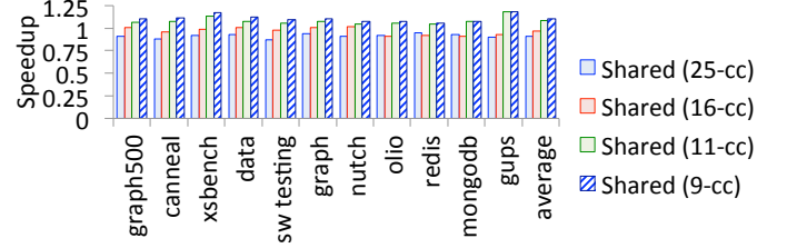
Fig. 4: Speedups using shared multi-banked TLBs over private L2 TLBs. Shared TLB access latencies varies from 25 to 9 cycles.
