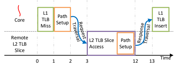
Fig. 10: Timeline of a virtual address translation in case of an L1 TLB miss and remote L2 TLB access in NOCSTAR.
